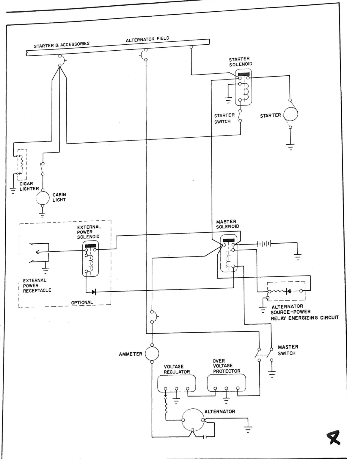
Alternator and Starter Schematic (Ser. Nos. 7415001 through 7415731)
